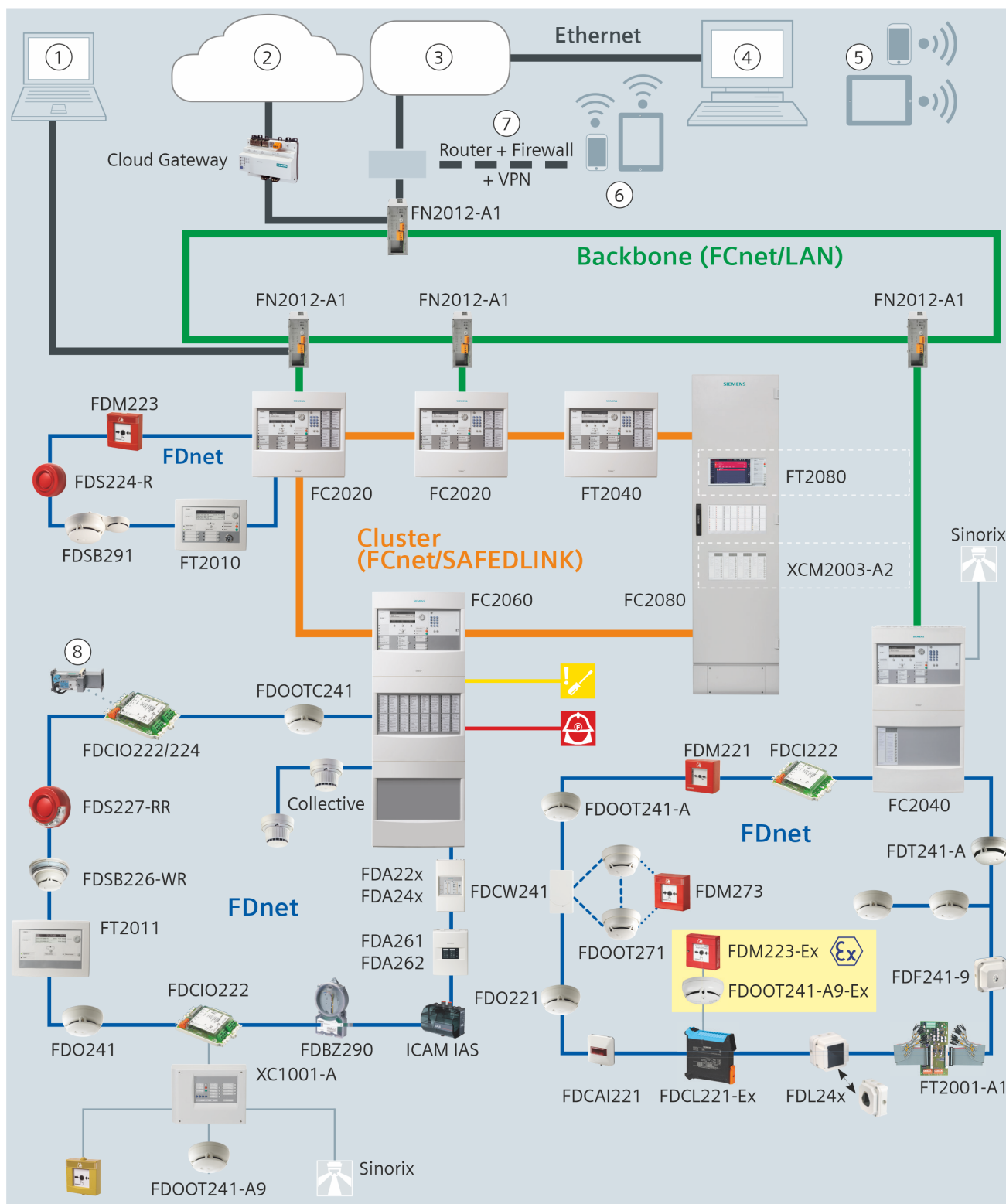
Fig. 1: System overview
